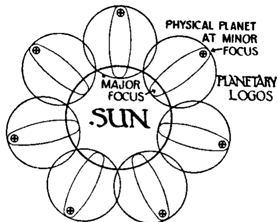
DIAGRAM XII.—Relation of Physical Planets to the Sun.
